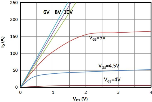
Fig 1: Output Characteristics
