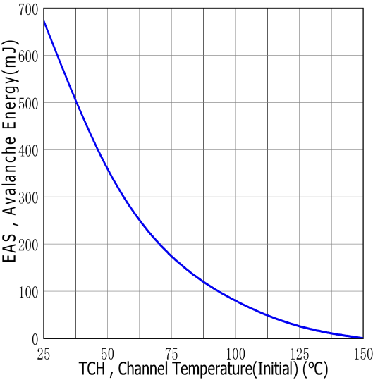
Figure.9 Maximum EAS vs Channel Temperature
