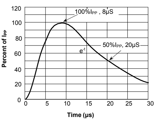
Fig.3 Pulse Waveform-8/20μs
