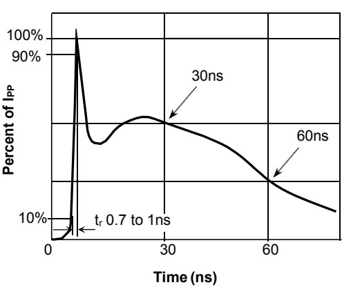
Fig.4 Pulse Waveform-ESD(IEC61000-4-2)
