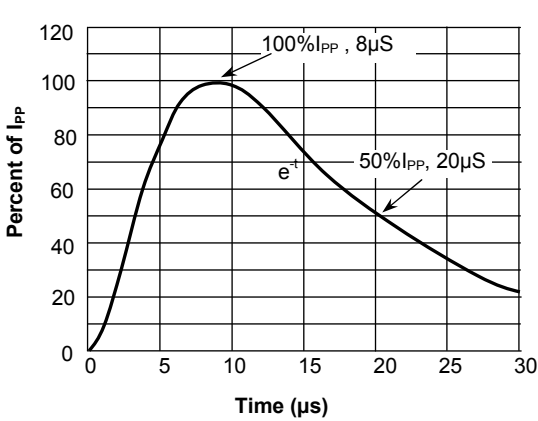
Fig.3 Pulse Waveform-8/20μs
