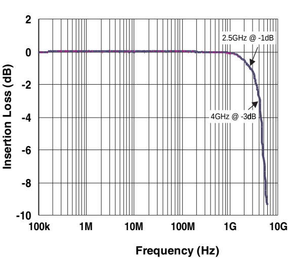
Fig.6 Insertion Loss S21 - I/O to GND
