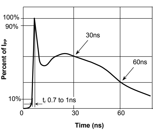
Fig.4 Pulse Waveform-ESD(IEC61000-4-2)
