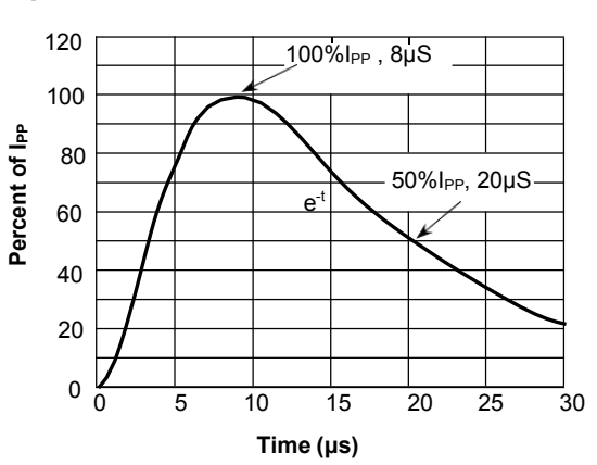
Fig.3 Pulse Waveform-8/20μs
