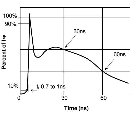
Fig.4 Pulse Waveform-ESD(IEC61000-4-2)
