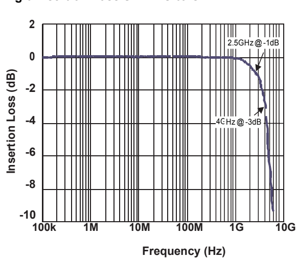
Fig.6 Insertion Loss S21 - I/O to GND
