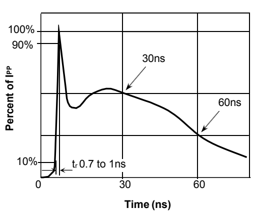
Fig.4 Pulse Waveform-ESD(IEC61000-4-2)
