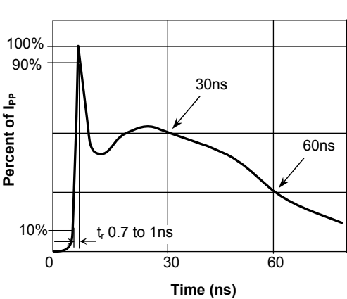
Fig.4 Pulse Waveform-ESD(IEC61000-4-2)
