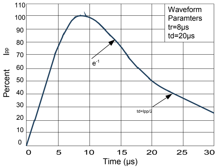
Figure3: Pulse Waveform
