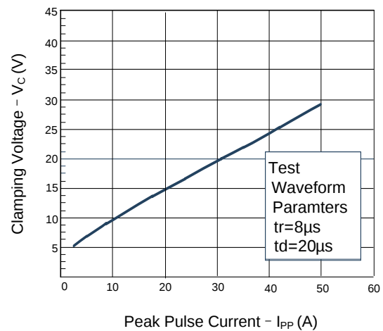
Figure 4: Clamping Voltage vs. I_pp
